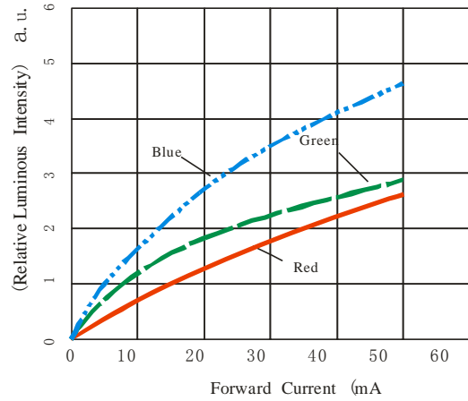
Relative Luminous Intensity VS Forward Current T Ambient 25
