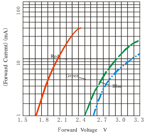
Volt-Ampere Characteristics T Ambient 25
